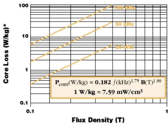
Core Loss vs. Flux Density† @ 25°C
